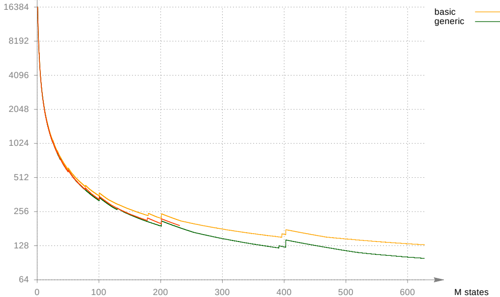
RSS per state, Tree compression, different visitors and number of threads
