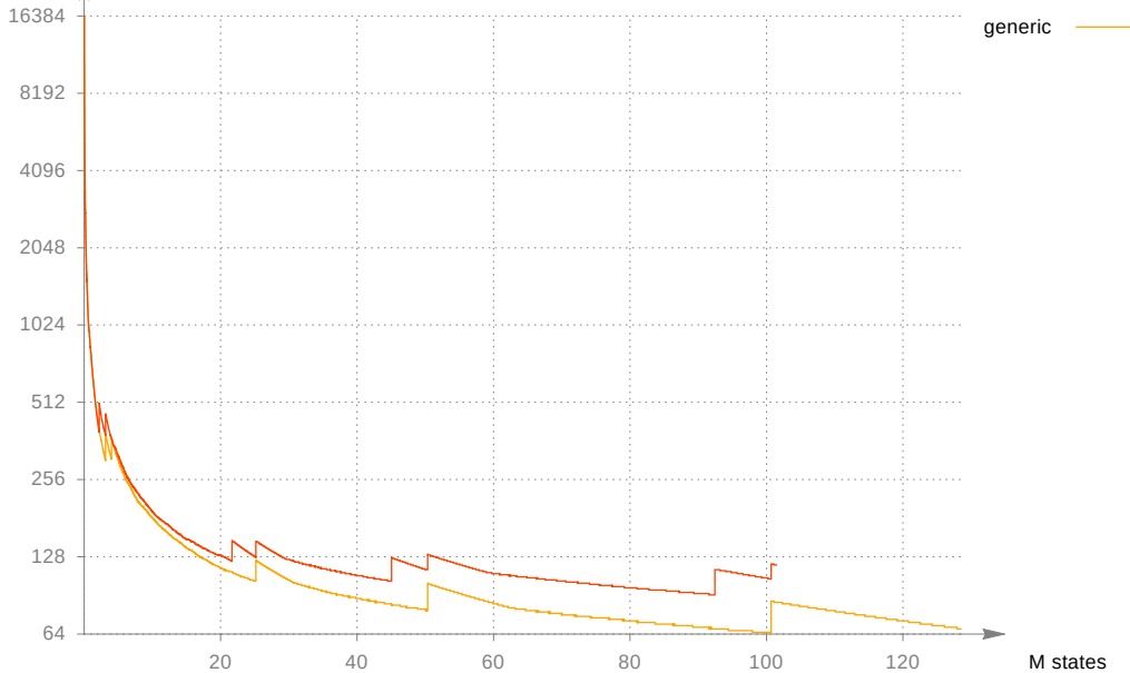
RSS per state, pthread_barrier, different splitters
